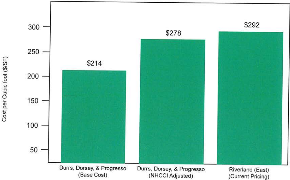
Cost per Cubic Foot of Installed Stormwater Conveyance (Before and After Inflation Adjustment)
