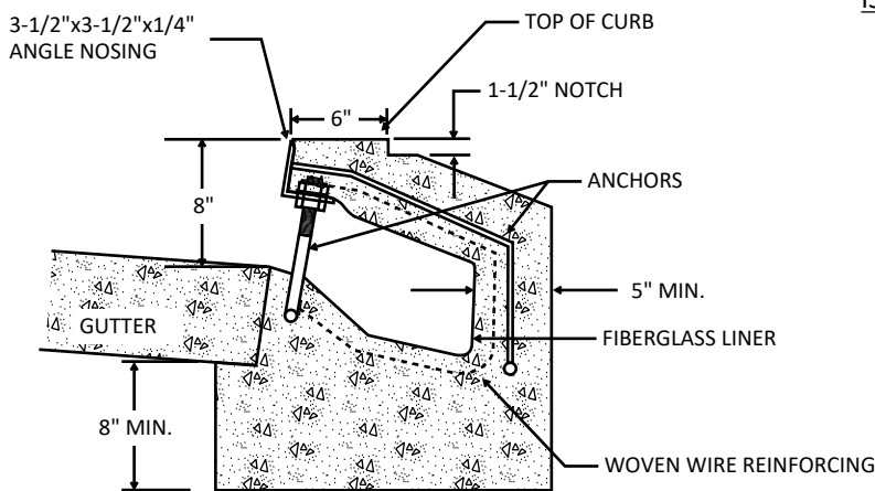
TYPICAL SECTION INSTALLED
