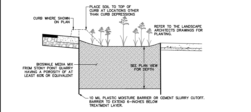
1 BIORETENTION AREA NO SCALE
